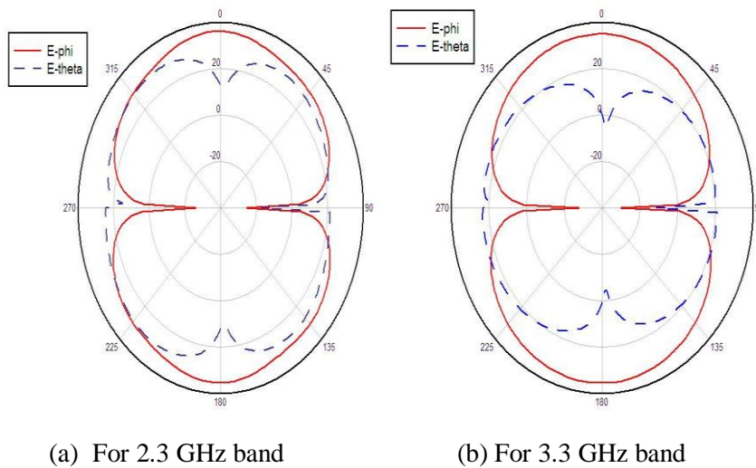
Figure 6 Radiation pattern of the proposed antenna.
