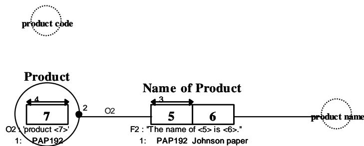
Figure 1 An example of IGD.
