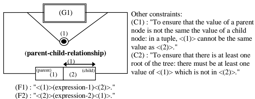
Figure 5 IG_{pD} for Parent-Child Pattern .
