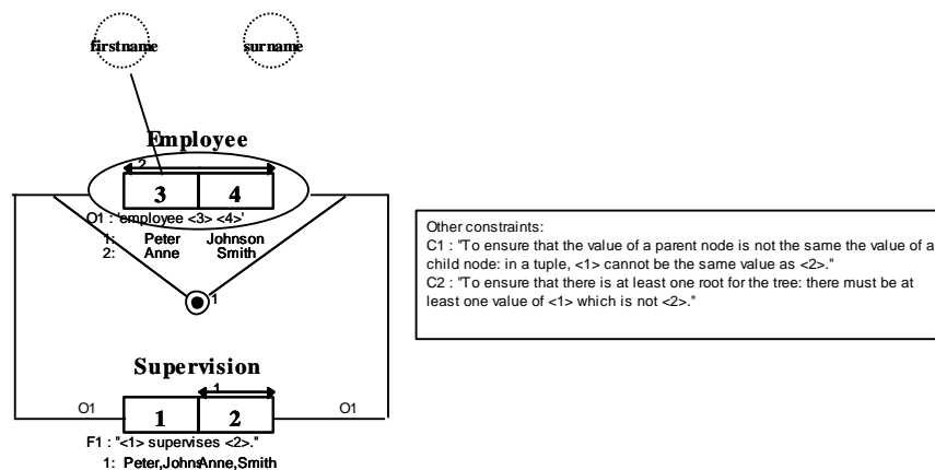
Figure 7 IGD for Supervision example based on the IG P D of Parent-Child Pattern .
