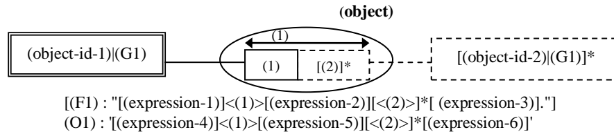
Figure 3 An example of IG P D.
