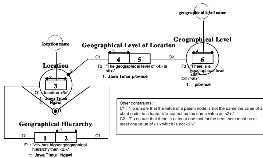
Figure 8 IGD for geographical location case study.
