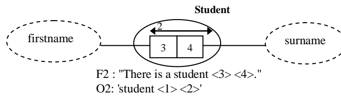
Figure 4 An example of an IGD generated based on the IG p and IG p D example.
