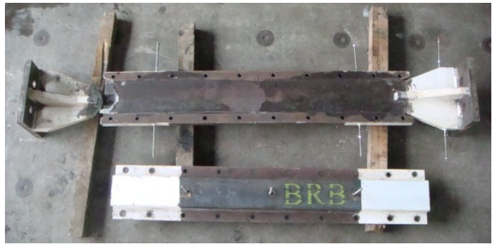
(b) Fracture (BRB 3, \epsilon_{max}=3.8\% )
