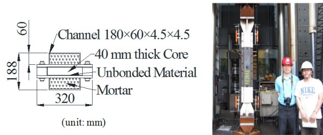
(a) BRBs 2-4
